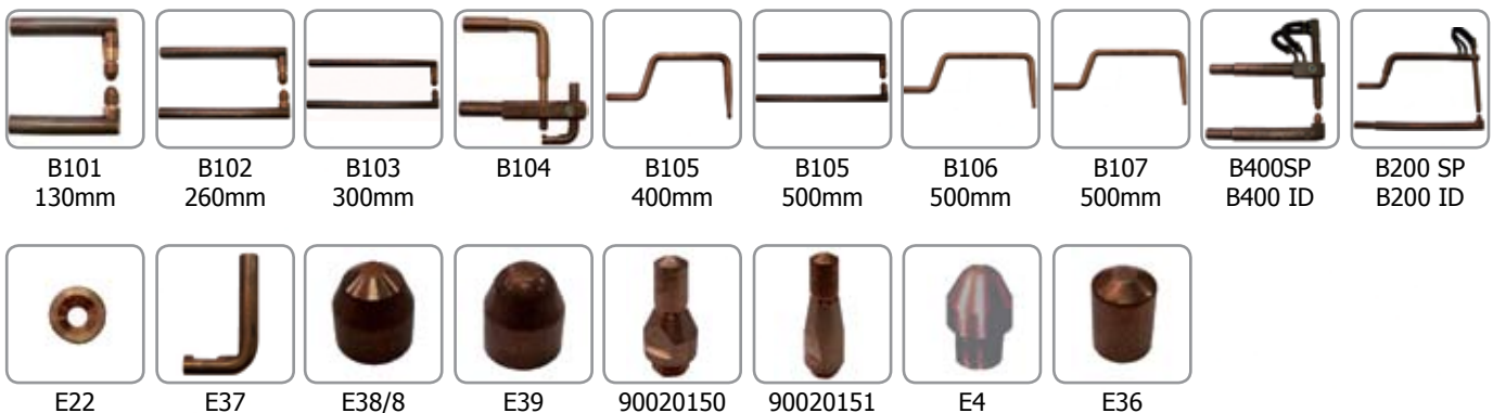
The X gun is available with 20mm cap electrodes or 13mm.
